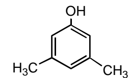
3,5-dimethylphenol
