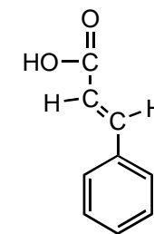
cinnamic acid
